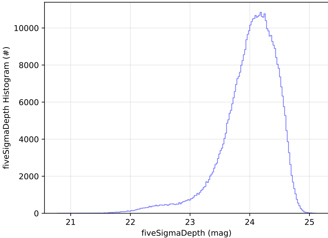
no_long_daily_v3.4_10yrs r: fiveSigmaDepth Histogram
