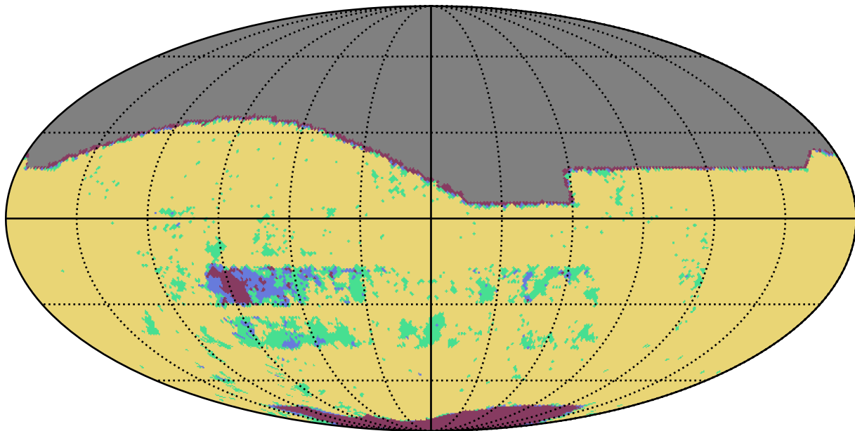
no_long_daily_v3.4_10yrs r band: YearCoverage night
