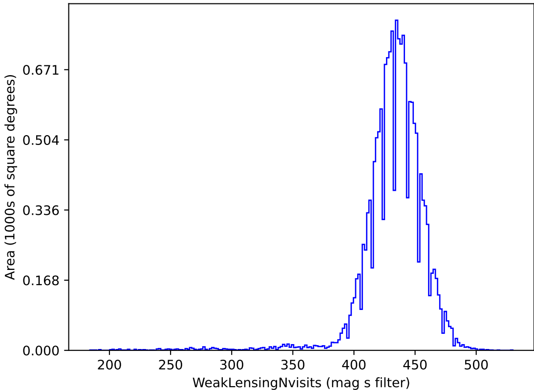
no_long_daily_v3.4_10yrs gri band non-DD: WeakLensingNvisits
