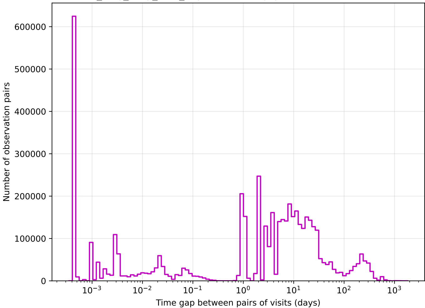
no_long_daily_v3.4_10yrs z band: Tgaps observationStartMJD
