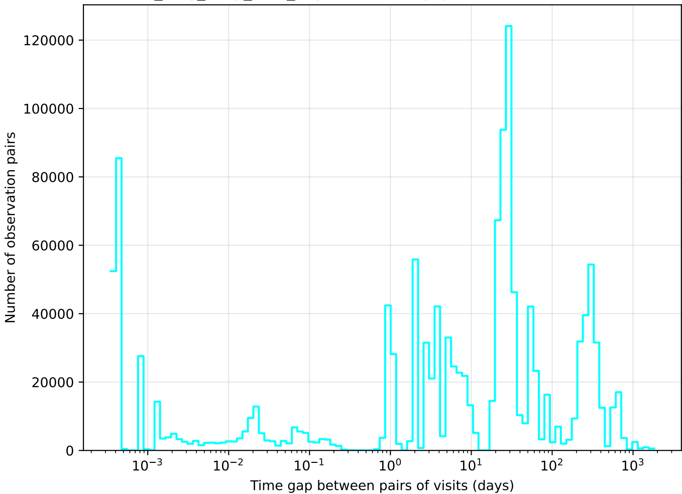
no_long_daily_v3.4_10yrs u band: Tgaps observationStartMJD
