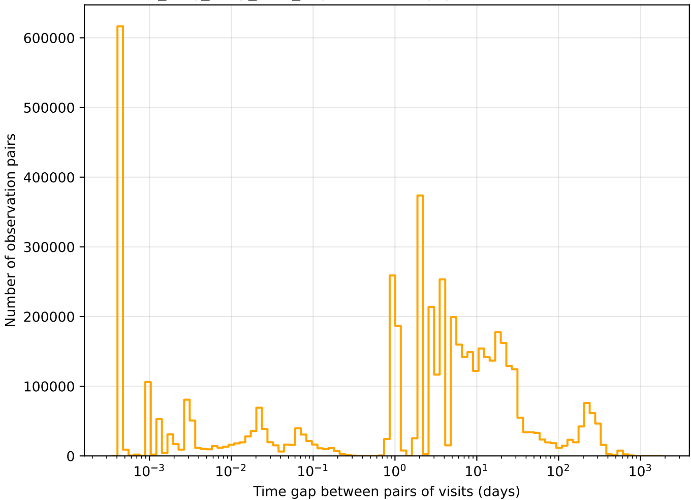
no_long_daily_v3.4_10yrs r band: Tgaps observationStartMJD
