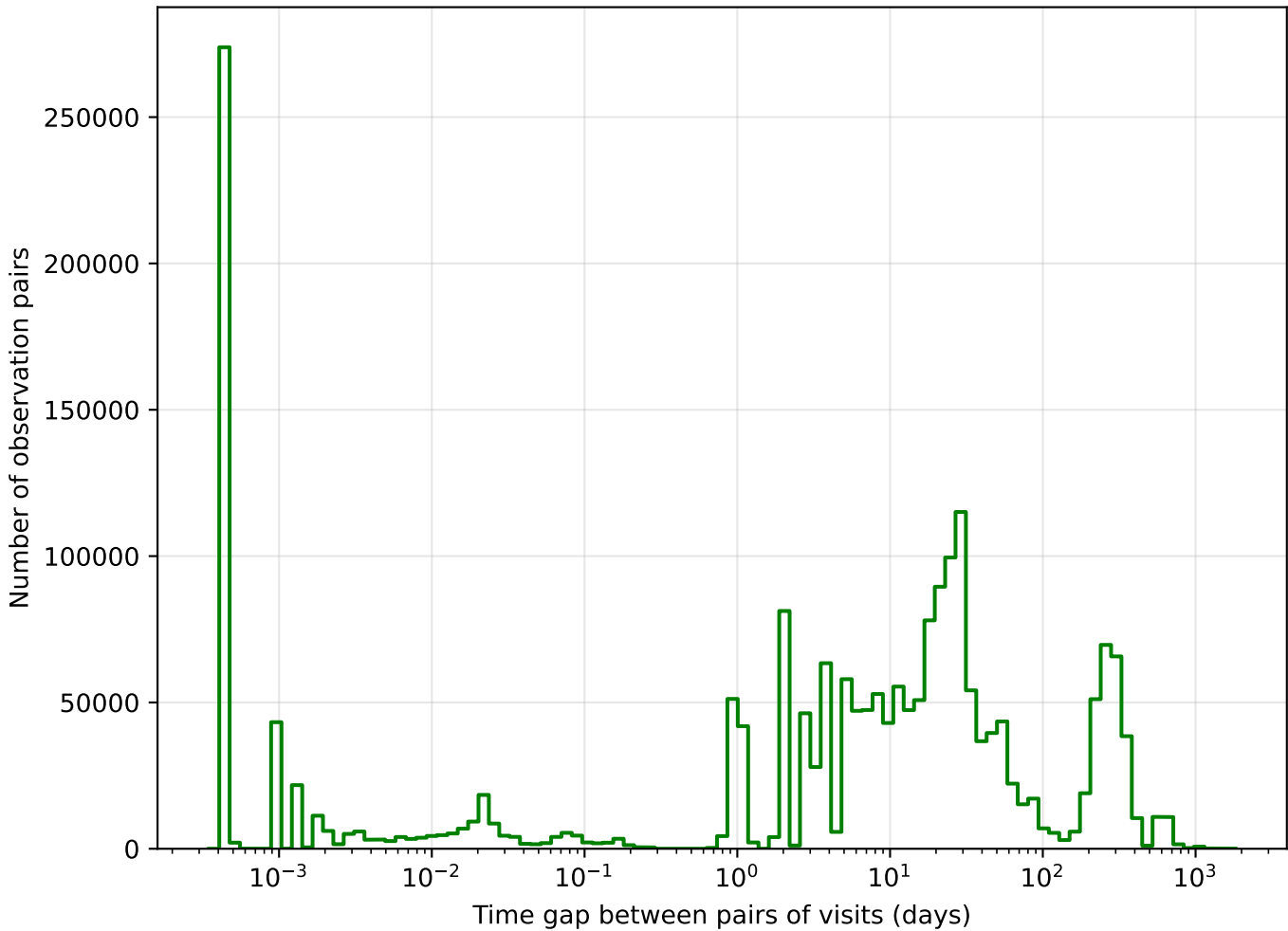
no_long_daily_v3.4_10yrs g band: Tgaps observationStartMJD
