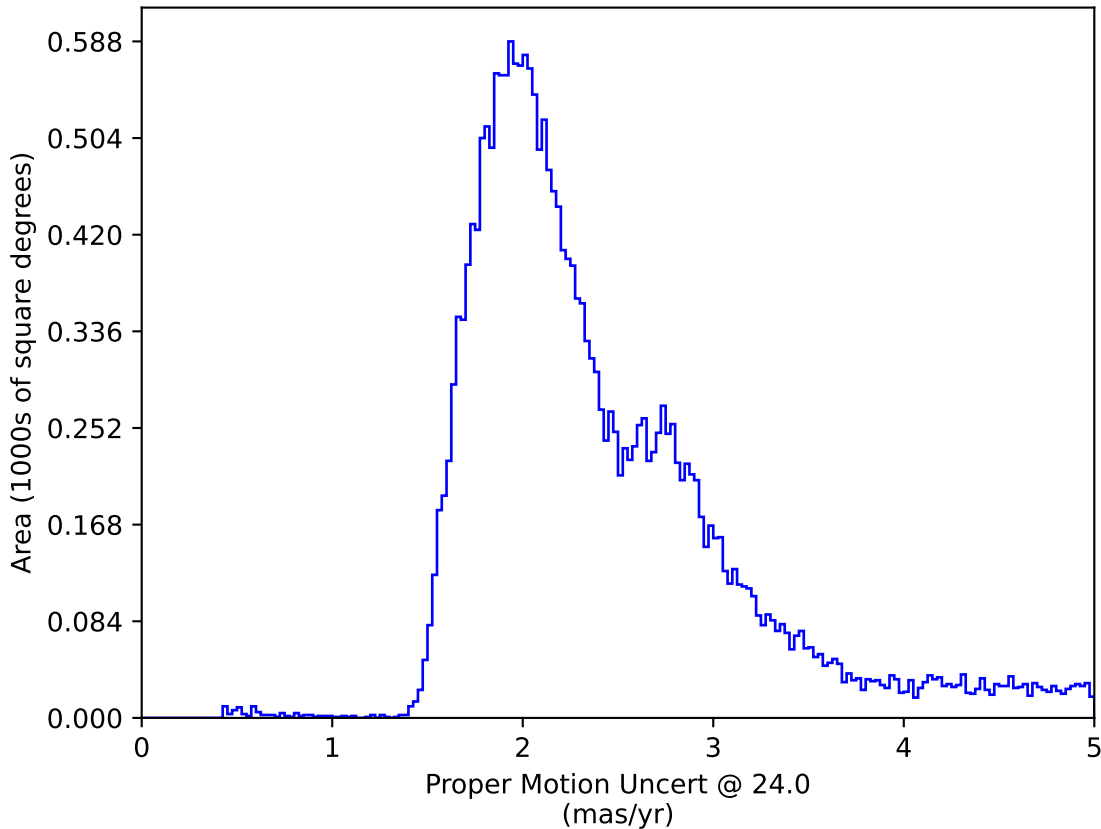
no_long_daily_v3.4_10yrs : Proper Motion Uncert @ 24.0
