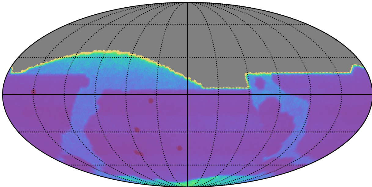
no_long_daily_v3.4_10yrs : Proper Motion Uncert @ 20.5
