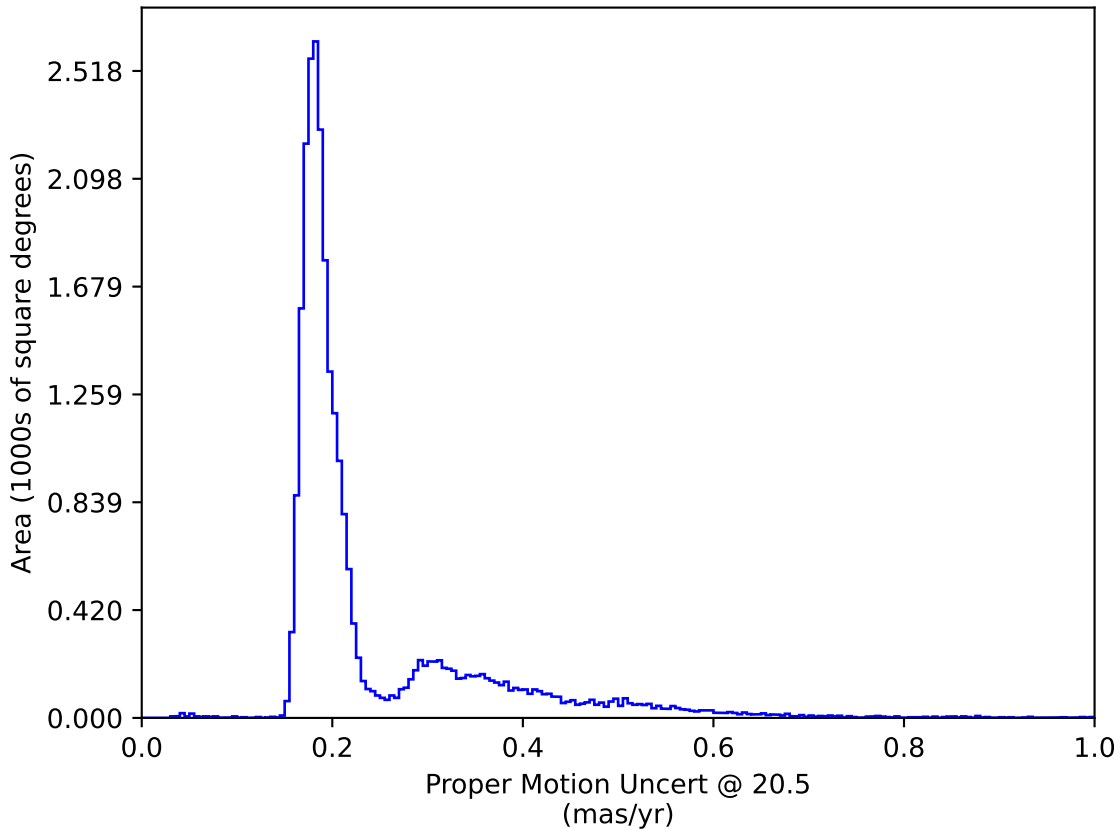
no_long_daily_v3.4_10yrs : Proper Motion Uncert @ 20.5
