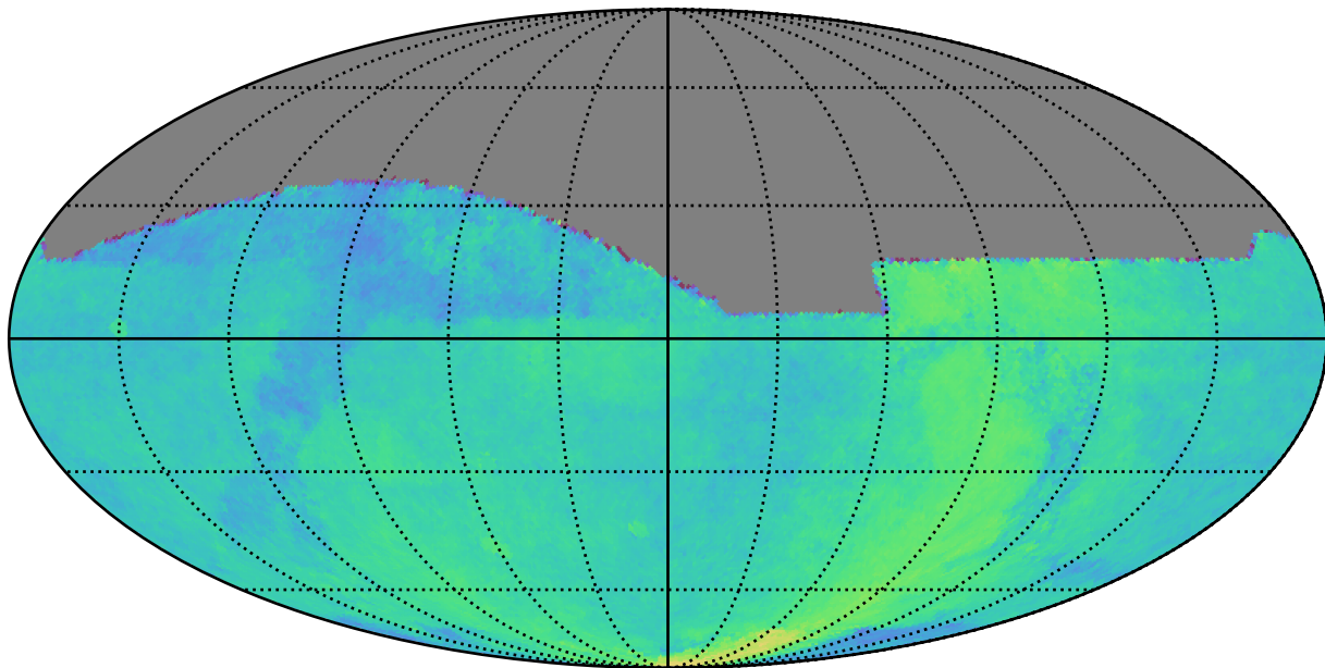
no_long_daily_v3.4_10yrs : Parallax Coverage @ 22.4
