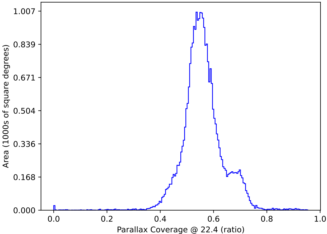
no_long_daily_v3.4_10yrs : Parallax Coverage @ 22.4
