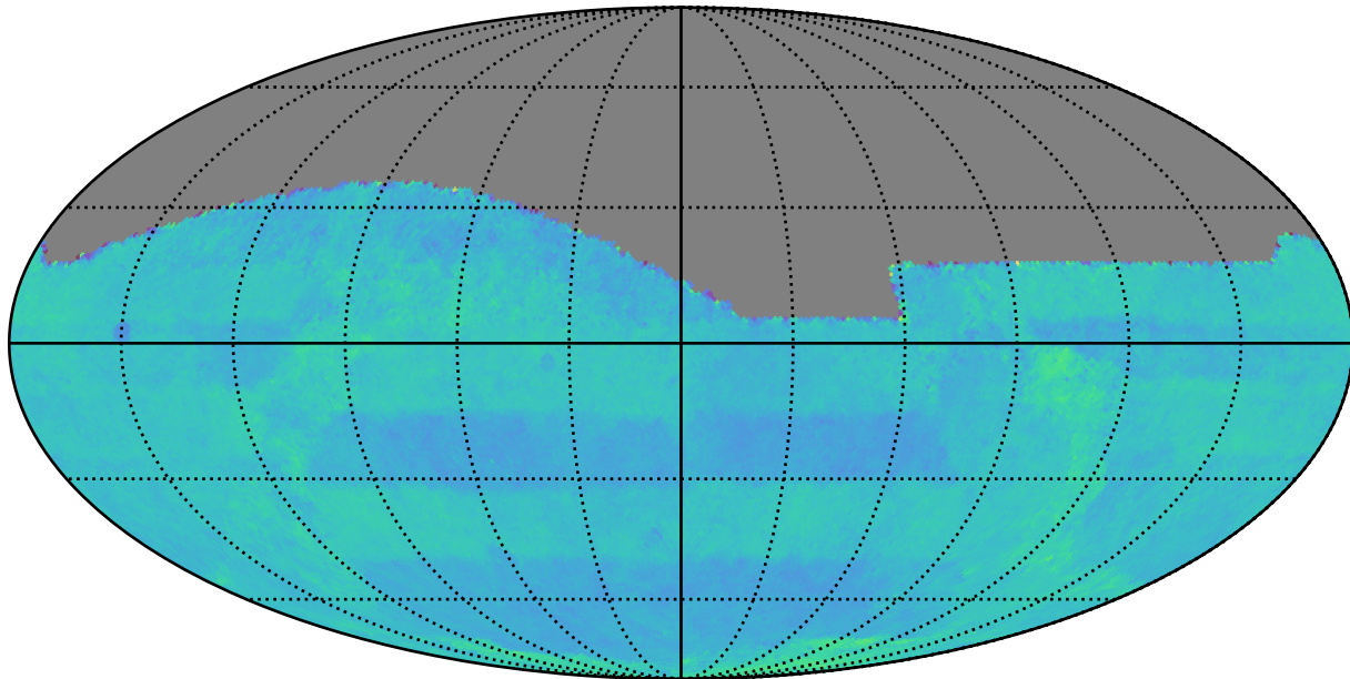
no_long_daily_v3.4_10yrs : Normalized Proper Motion Uncert @ 24.0
