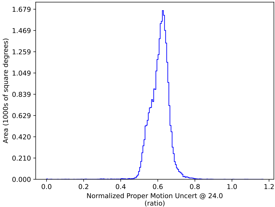
no_long_daily_v3.4_10yrs : Normalized Proper Motion Uncert @ 24.0
