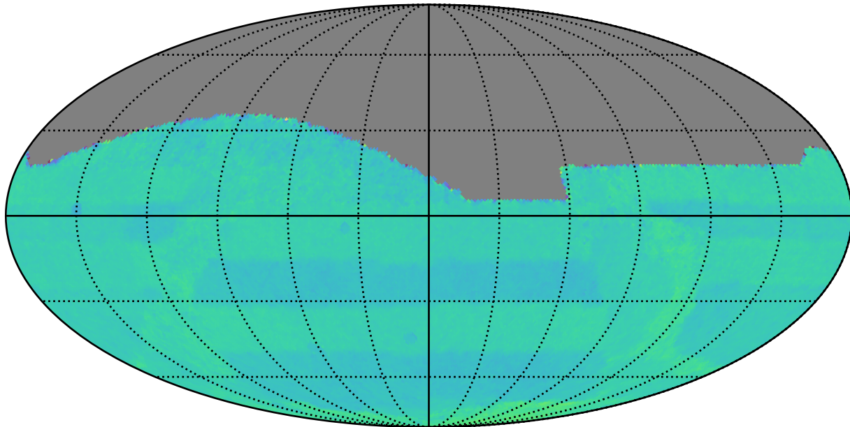
no_long_daily_v3.4_10yrs : Normalized Proper Motion Uncert @ 20.5
