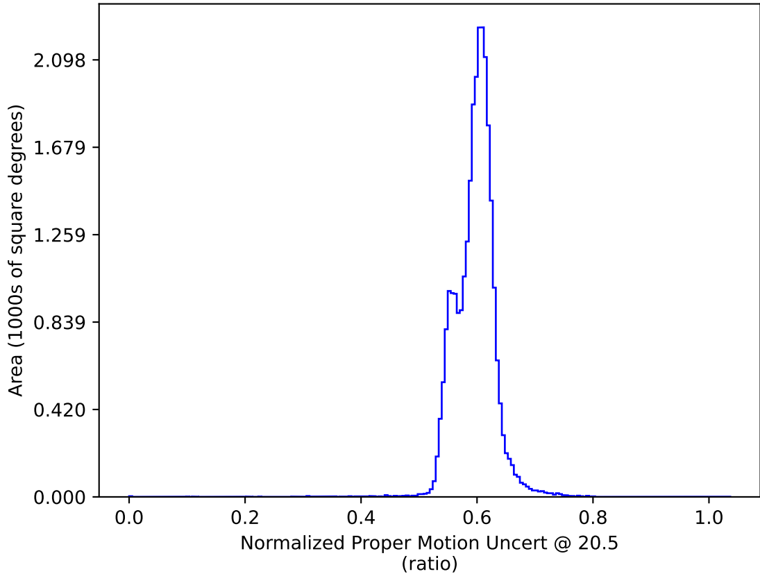
no_long_daily_v3.4_10yrs : Normalized Proper Motion Uncert @ 20.5
