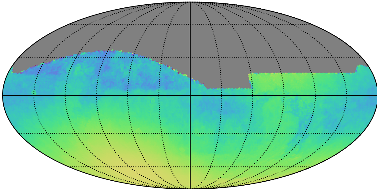
no_long_daily_v3.4_10yrs : Normalized Parallax Uncert @ 24.0
