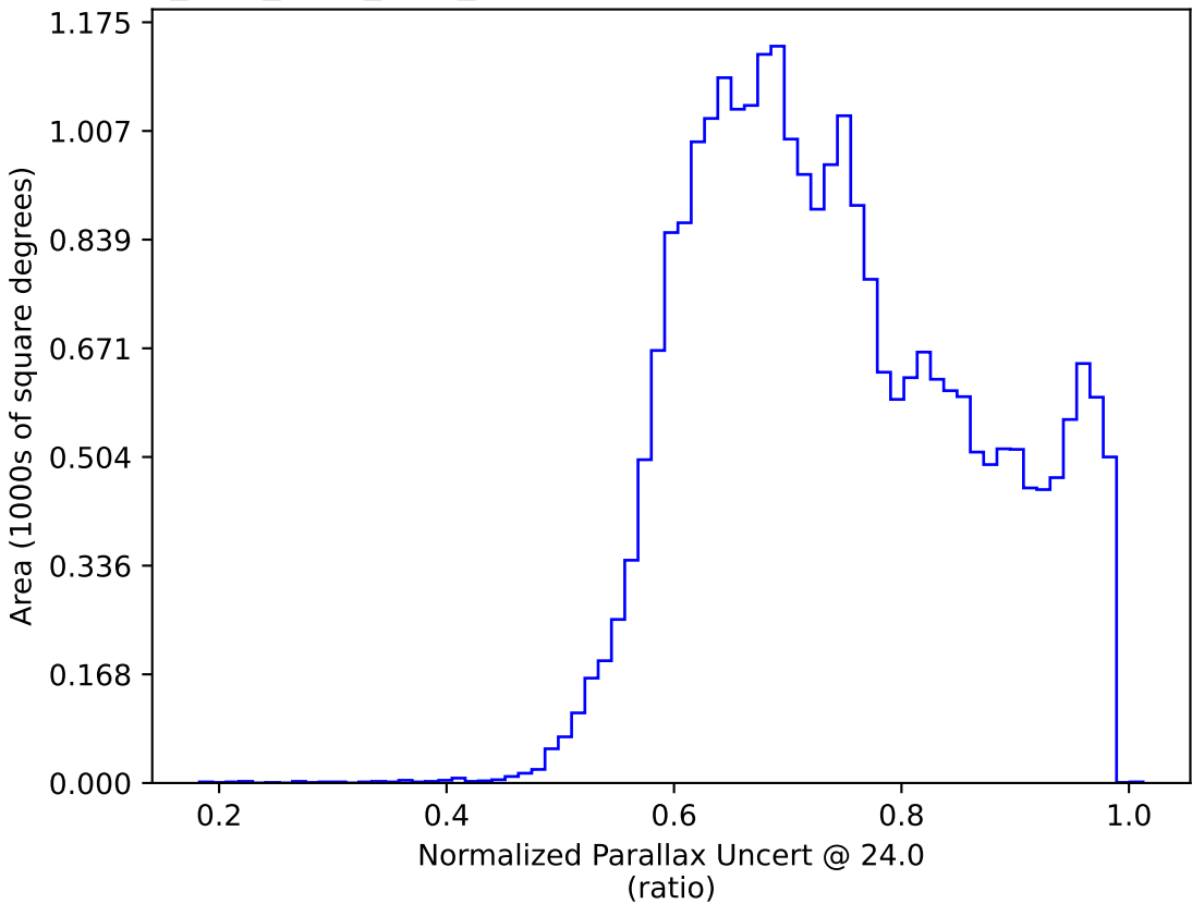
no_long_daily_v3.4_10yrs : Normalized Parallax Uncert @ 24.0
