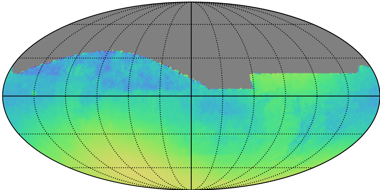
no_long_daily_v3.4_10yrs : Normalized Parallax Uncert @ 22.4
