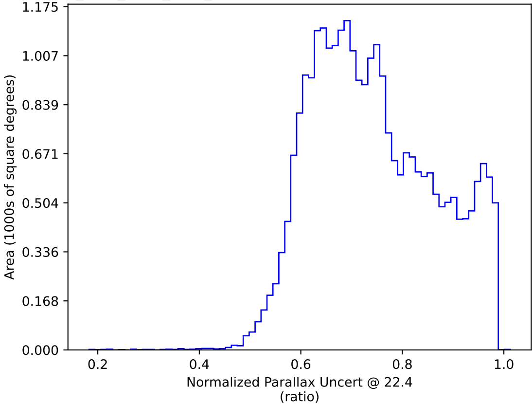
no_long_daily_v3.4_10yrs : Normalized Parallax Uncert @ 22.4
