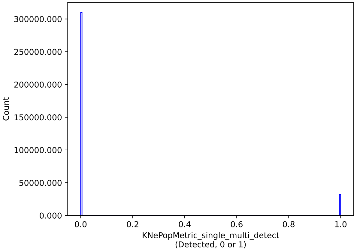
no_long_daily_v3.4_10yrs single model: KNePopMetric_single_multi_detect
