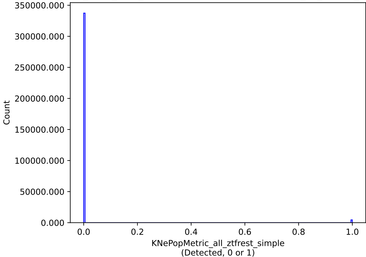
no_long_daily_v3.4_10yrs all models: KNePopMetric_all_ztfrest_simple
