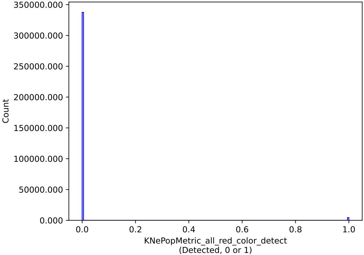
no_long_daily_v3.4_10yrs all models: KNePopMetric_all_red_color_detect
