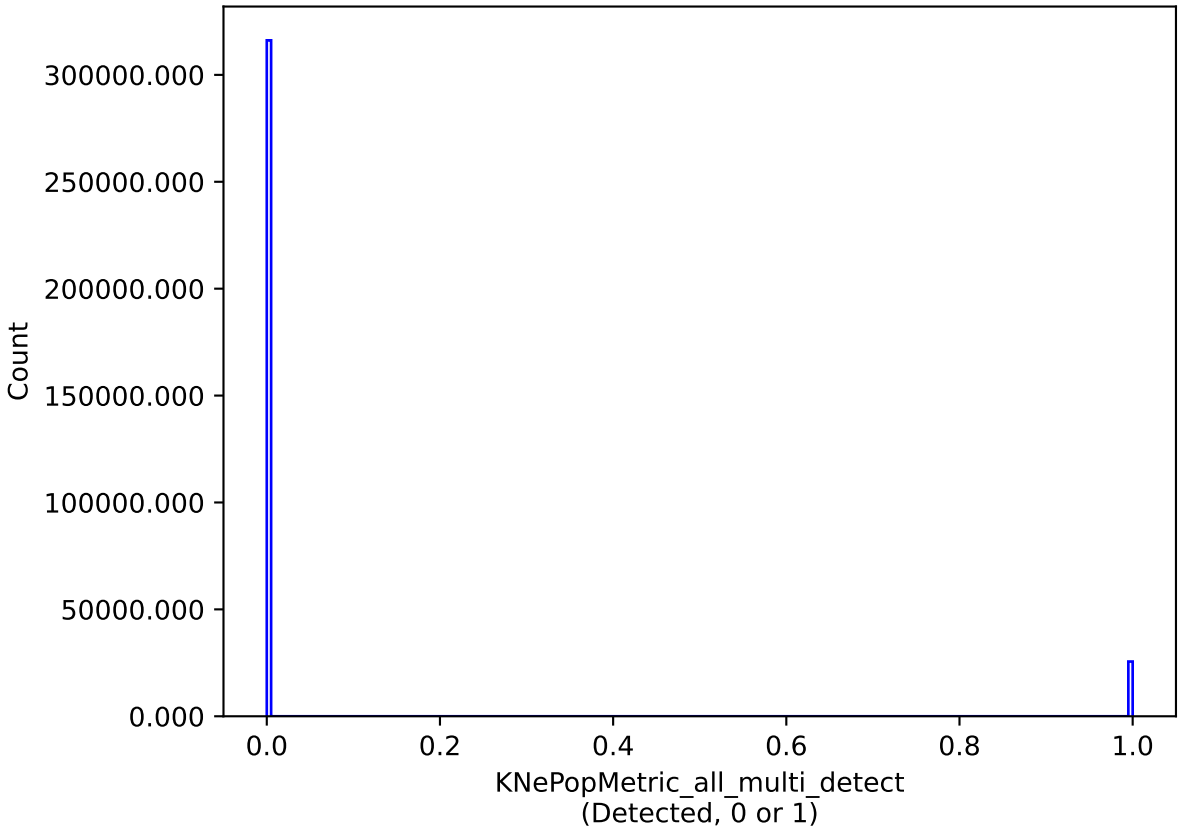
no_long_daily_v3.4_10yrs all models: KNePopMetric_all_multi_detect
