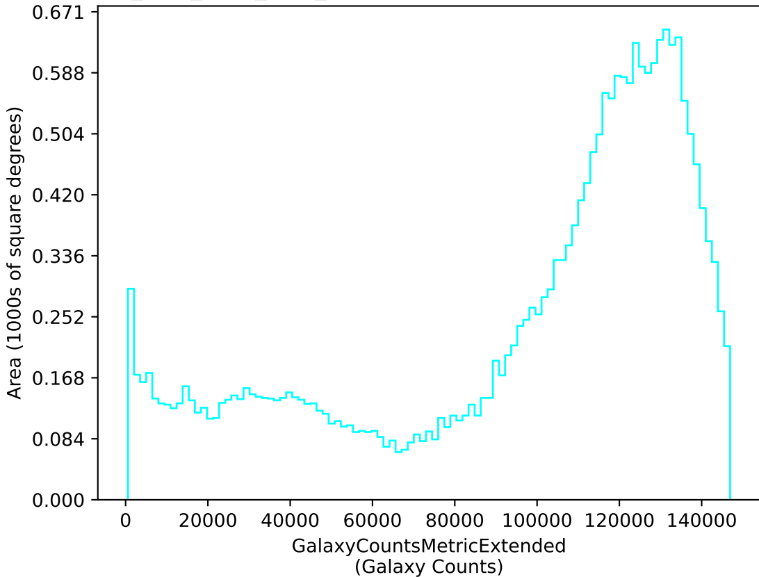
no_long_daily_v3.4_10yrs u: GalaxyCountsMetricExtended
