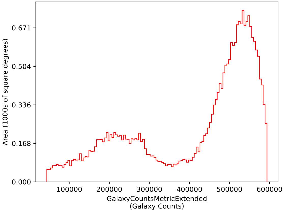
no_long_daily_v3.4_10yrs i: GalaxyCountsMetricExtended
