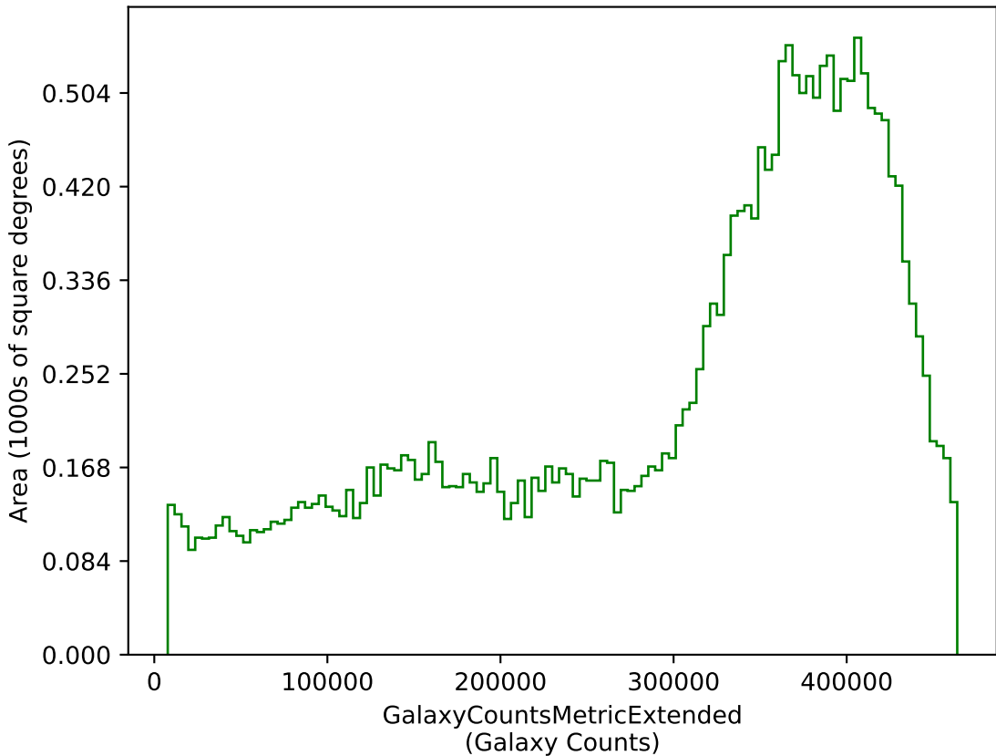
no_long_daily_v3.4_10yrs g: GalaxyCountsMetricExtended
