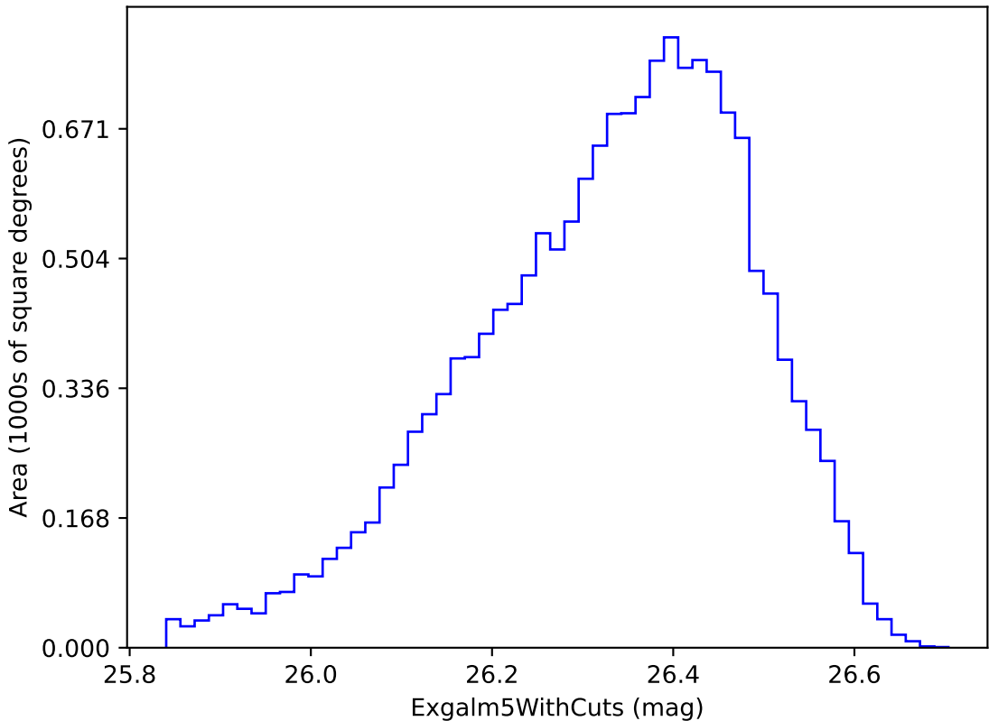
no_long_daily_v3.4_10yrs i band non-DD year 9: Exgal5WithCuts
