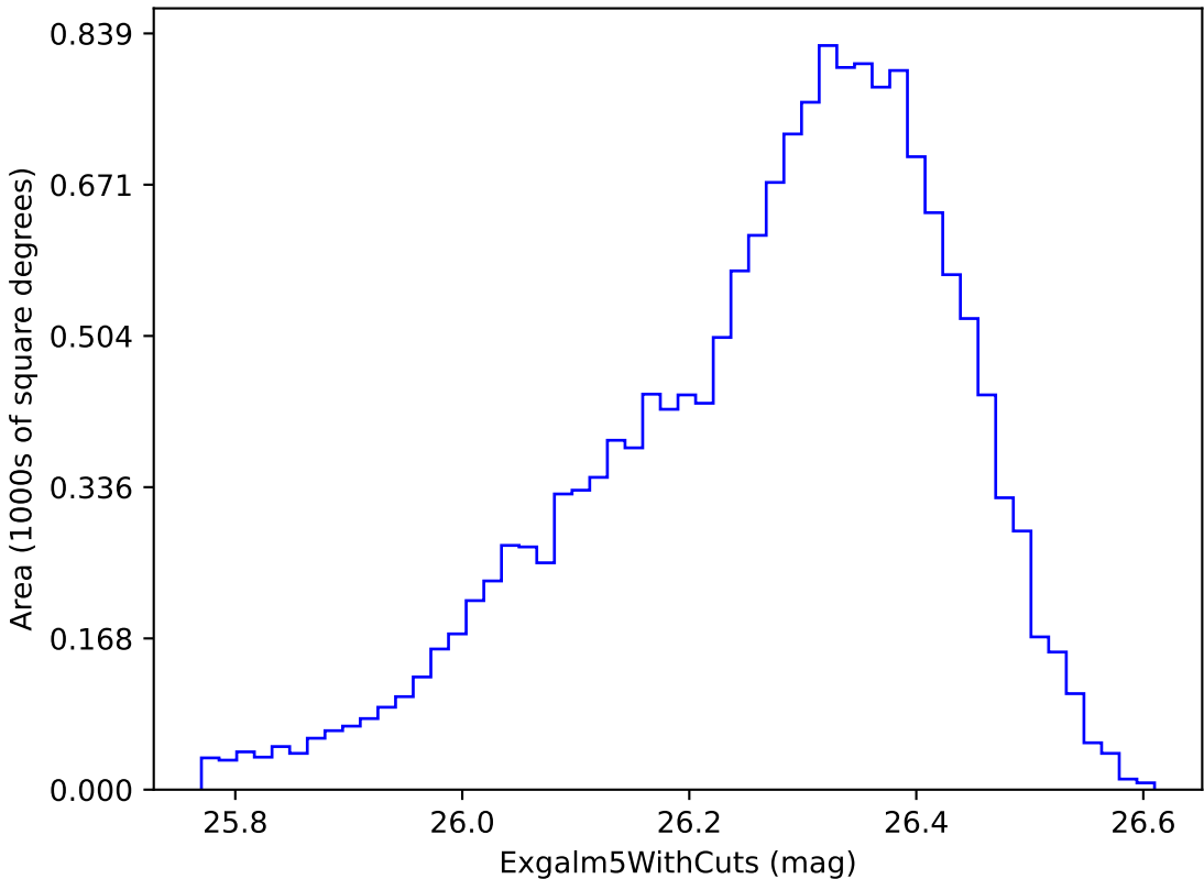
no_long_daily_v3.4_10yrs i band non-DD year 8: Exgalml5WithCuts
