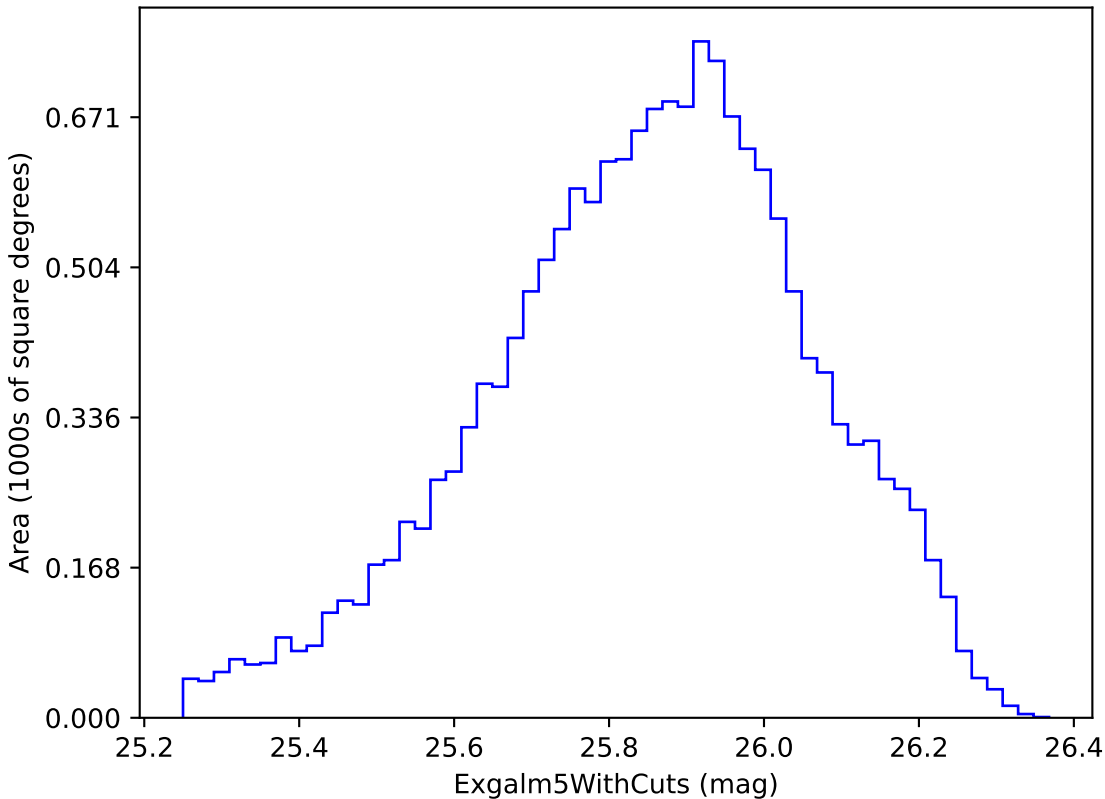
no_long_daily_v3.4_10yrs i band non-DD year 3: Exgal5WithCuts
