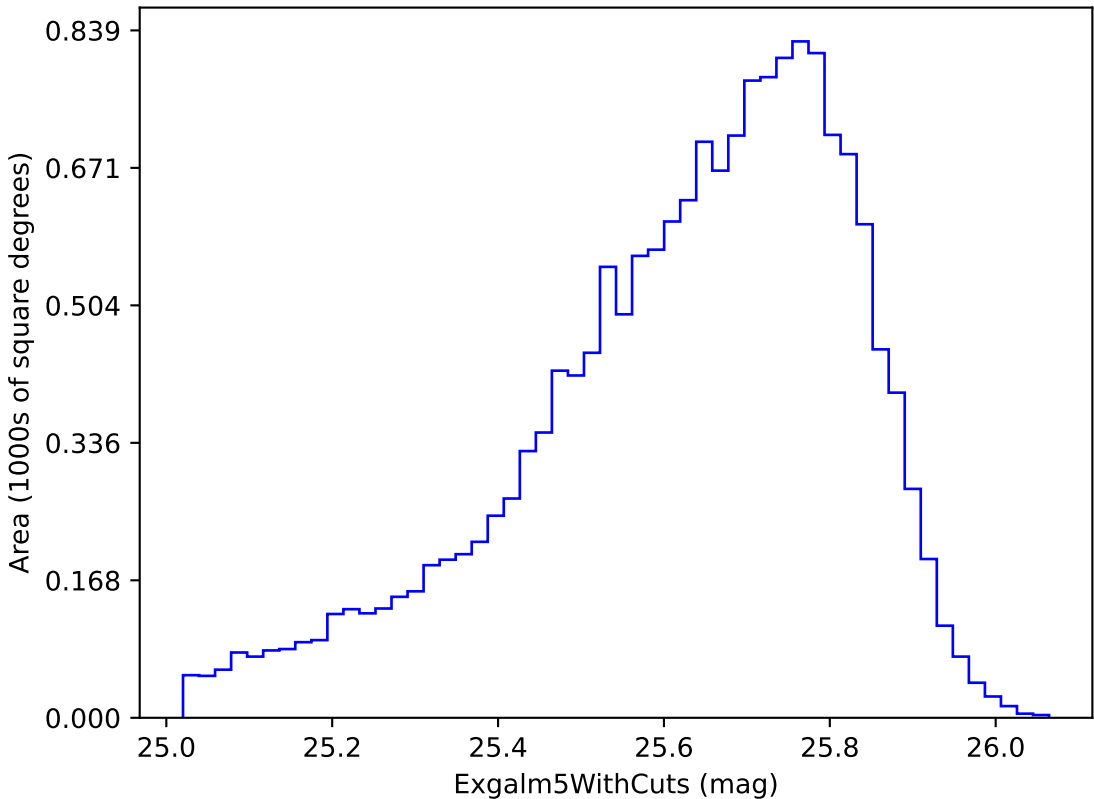
no_long_daily_v3.4_10yrs i band non-DD year 2: Exgal5WithCuts
