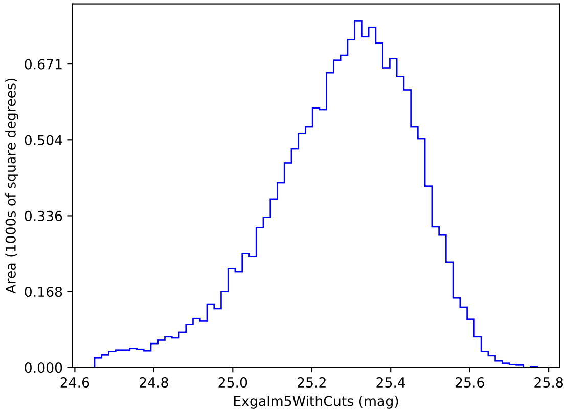
no_long_daily_v3.4_10yrs i band non-DD year 1: Exgalml5WithCuts
