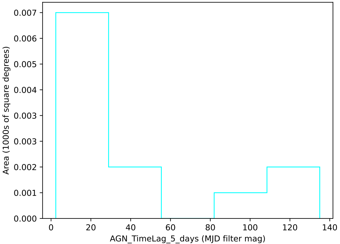
no_long_daily_v3.4_10yrs u band: AGN_TimeLag_5_days
