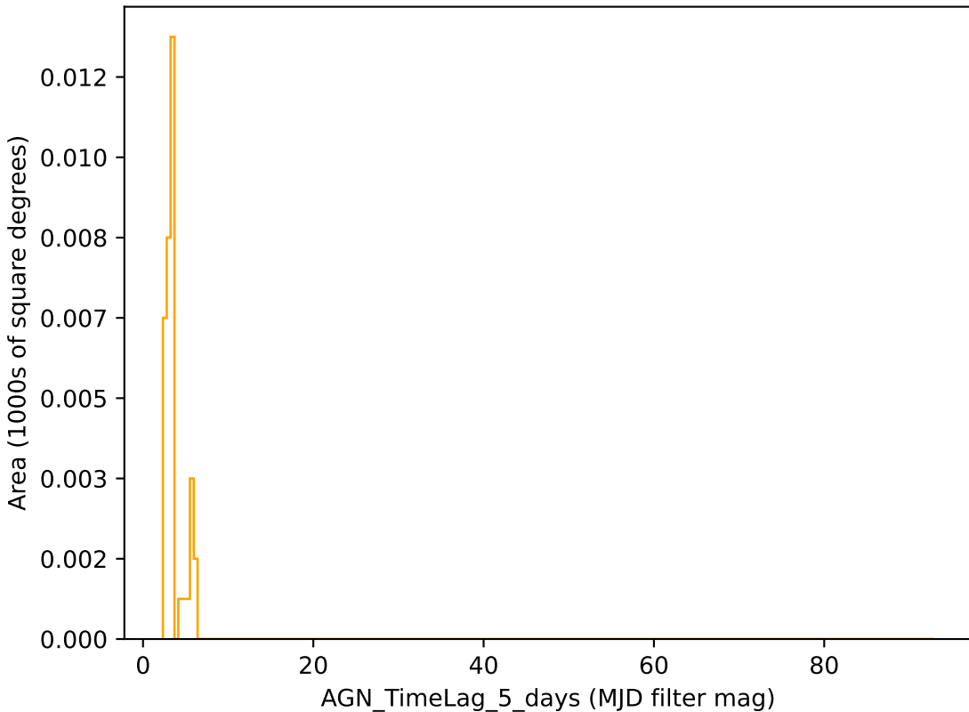
no_long_daily_v3.4_10yrs r band: AGN_TimeLag_5_days
