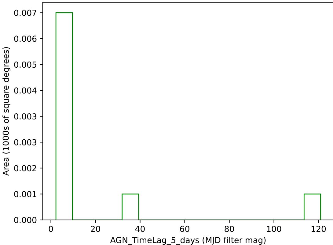
no_long_daily_v3.4_10yrs g band: AGN_TimeLag_5_days
