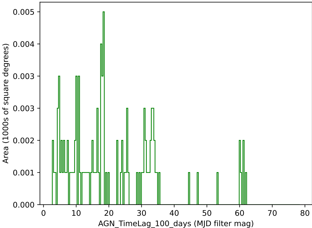
no_long_daily_v3.4_10yrs g band: AGN_TimeLag_100_days
