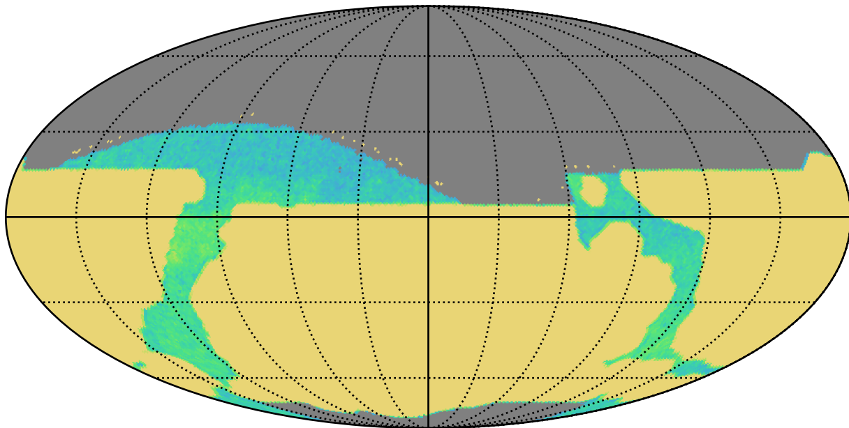
no_long_daily_v3.4_10yrs all bands: AGN_TimeLag_100_days
