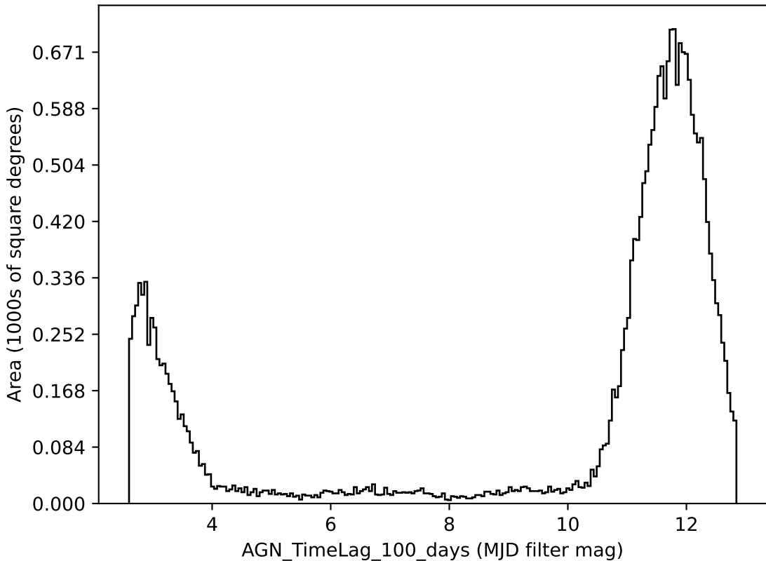
no_long_daily_v3.4_10yrs all bands: AGN_TimeLag_100_days
