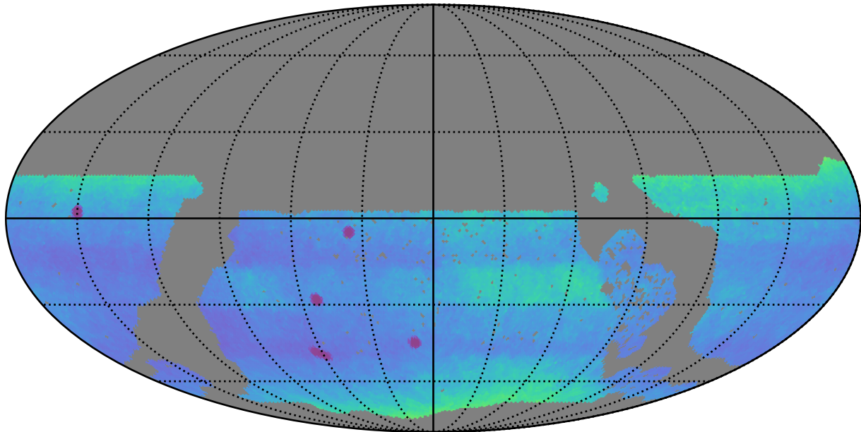
no_long_daily_v3.4_10yrs WFD: Proper Motion Uncert @ 24.0
