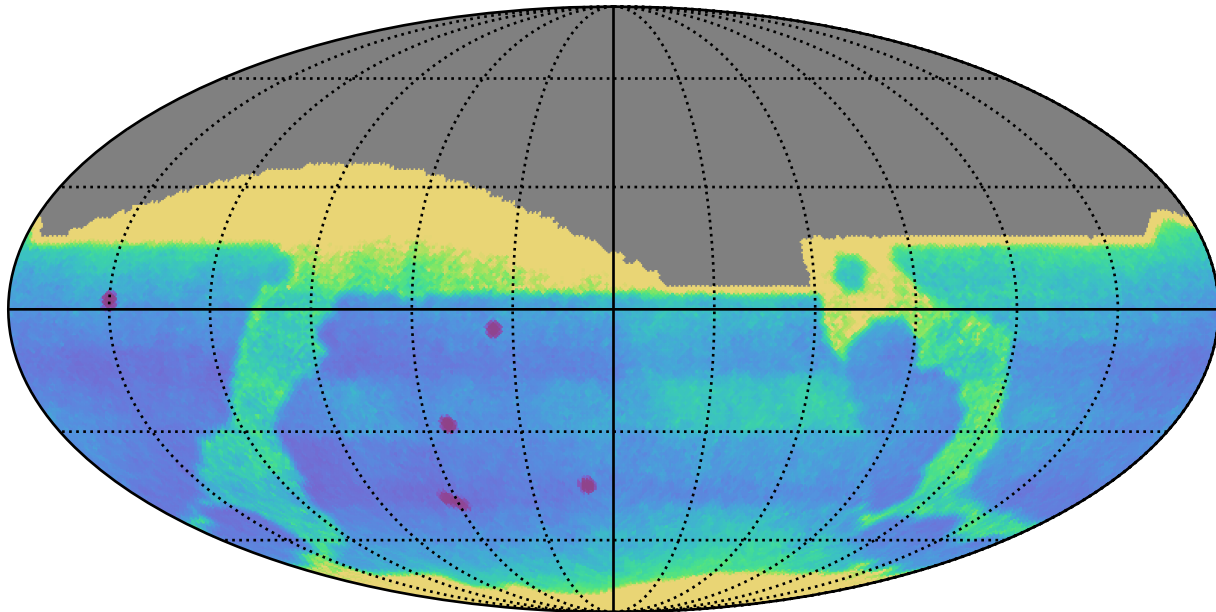
no_long_daily_v3.4_10yrs All sky: Proper Motion Uncert @ 24.0
