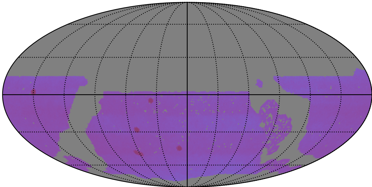
no_long_daily_v3.4_10yrs WFD: Proper Motion Uncert @ 20.5
