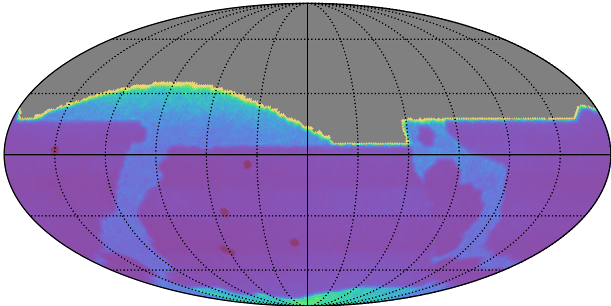
no_long_daily_v3.4_10yrs All sky: Proper Motion Uncert @ 20.5
