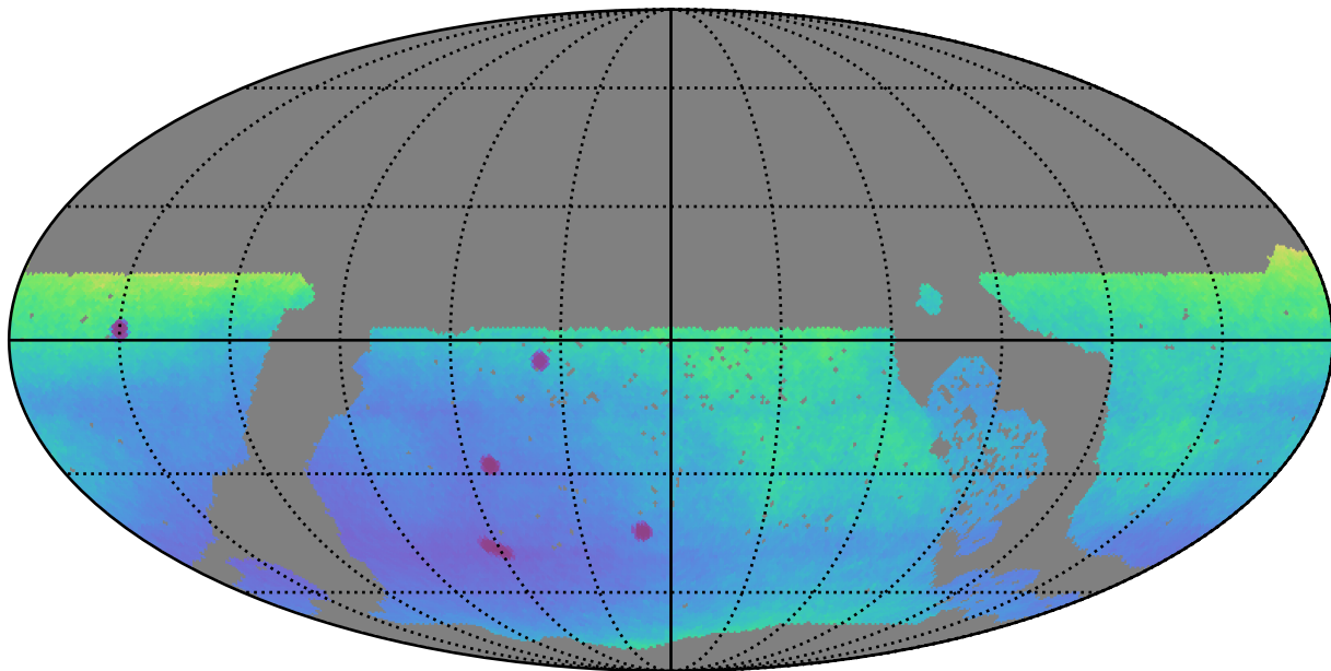
no_long_daily_v3.4_10yrs WFD: Parallax Uncert @ 24.0
