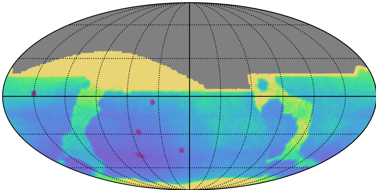
no_long_daily_v3.4_10yrs All sky: Parallax Uncert @ 22.4
