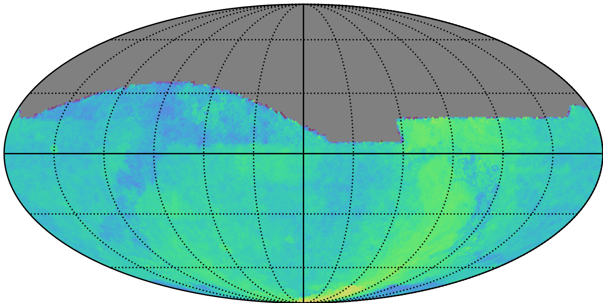
no_long_daily_v3.4_10yrs All sky: Parallax Coverage @ 24.0
