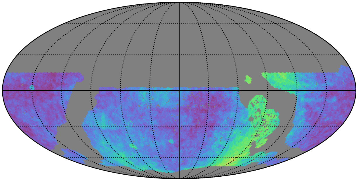
no_long_daily_v3.4_10yrs WFD: Parallax Coverage @ 22.4
