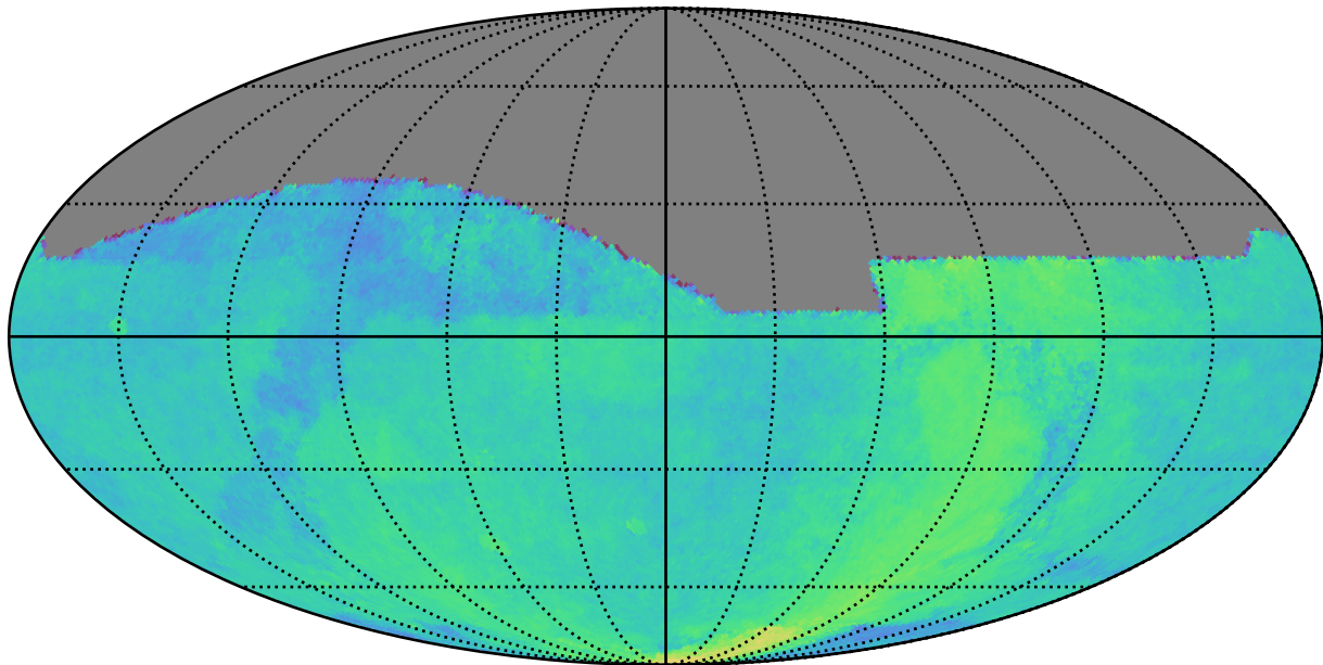
no_long_daily_v3.4_10yrs All sky: Parallax Coverage @ 22.4
