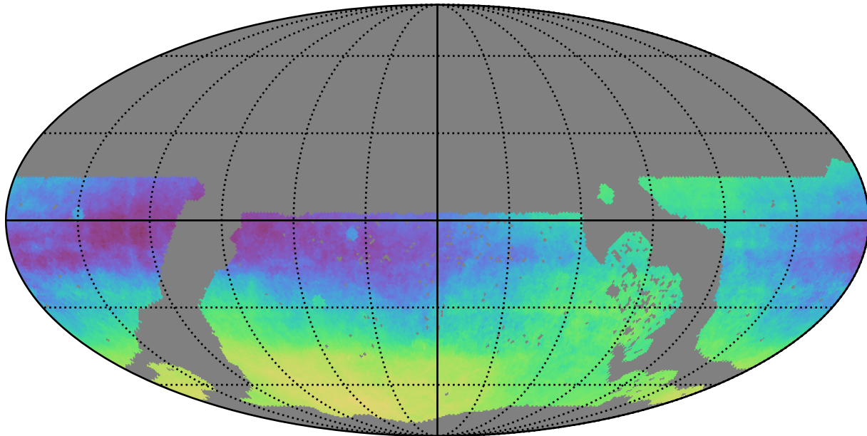
no_long_daily_v3.4_10yrs WFD: Parallax-DCR degeneracy @ 22.4
