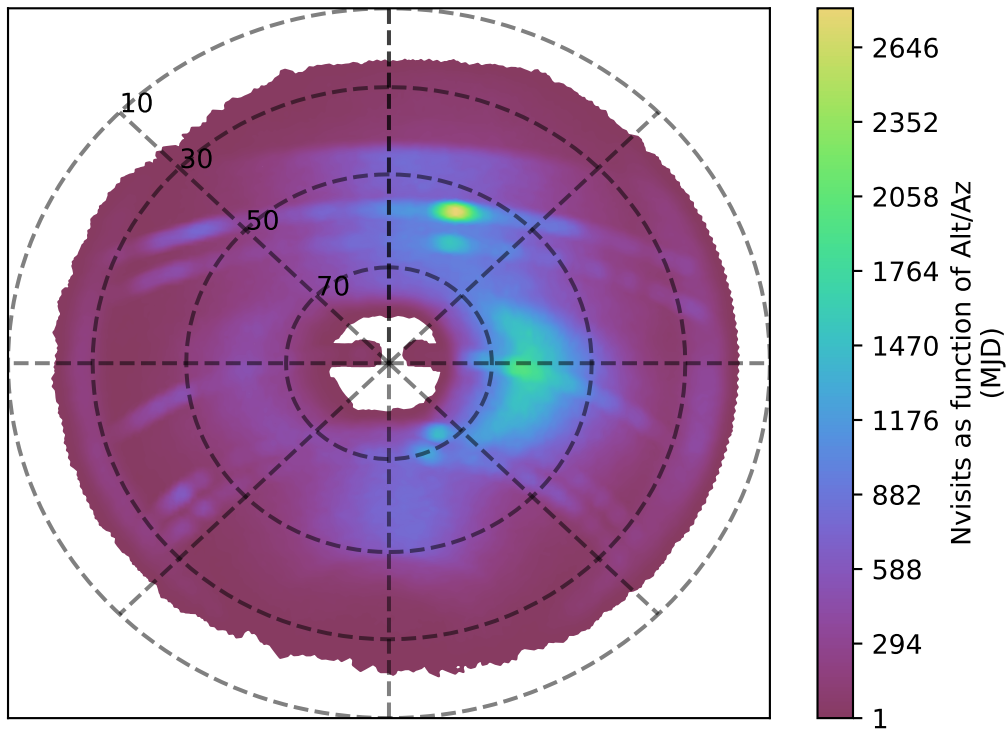
no_long_daily_v3.4_10yrs z band: Nvisits as function of Alt/Az
