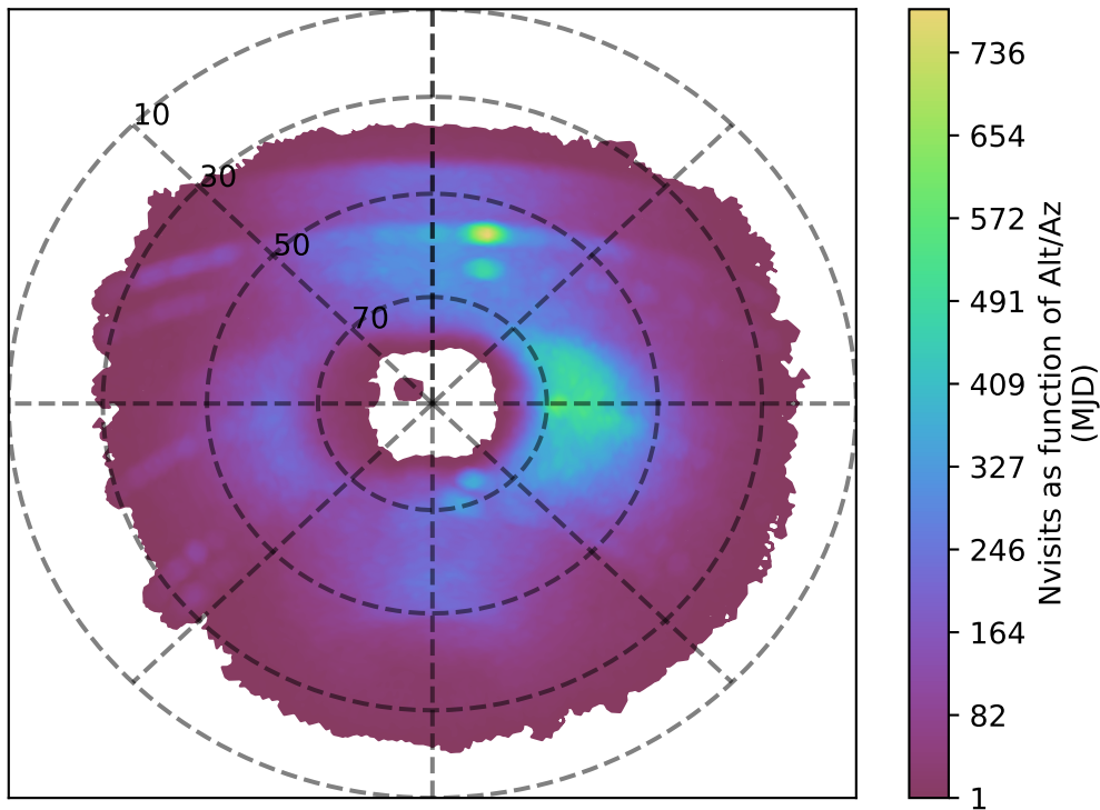
no_long_daily_v3.4_10yrs u band: Nvisits as function of Alt/Az
